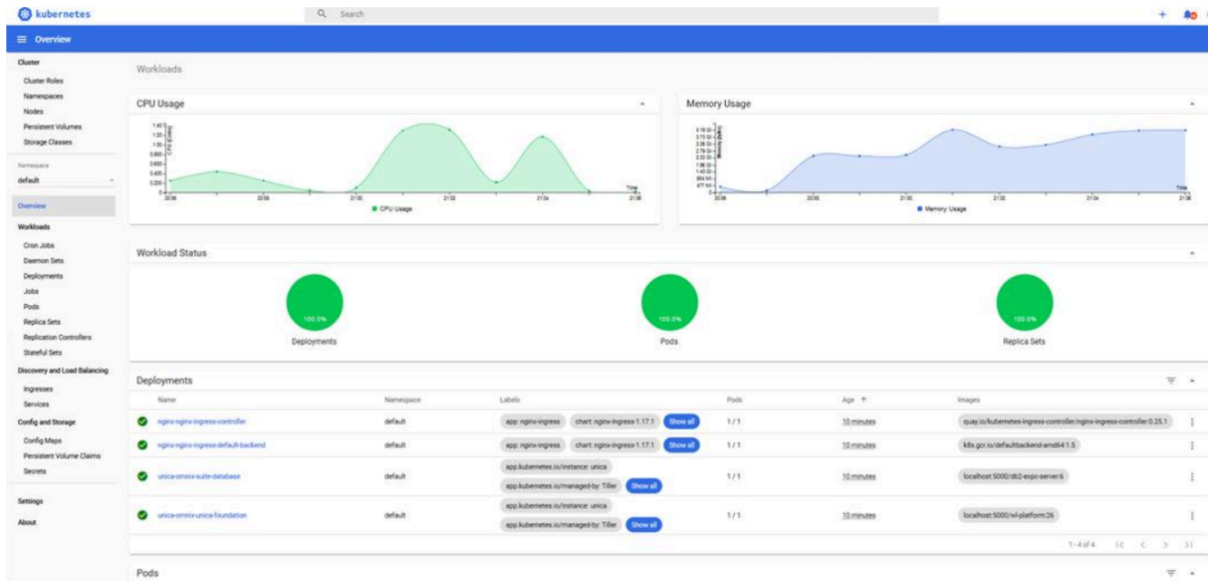
Figure 1. Kubernetes dashboard
