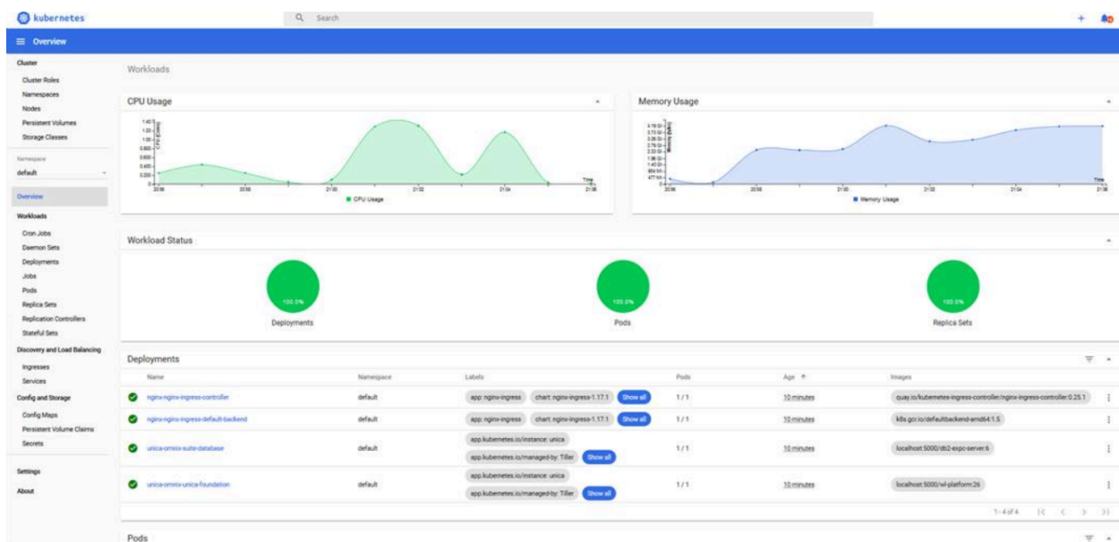
Figure 1. Kubernetes dashboard
