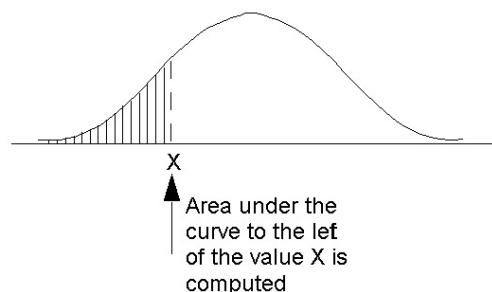
Area Under a Gaussian Computed by GAUSS_AREA
